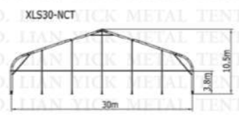
30m & 40m New Curve Aluminium technology tent
