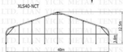
30m & 40m New Curve Aluminium technology tent
