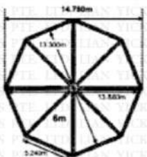
OCTAGON TRUSS TENT
